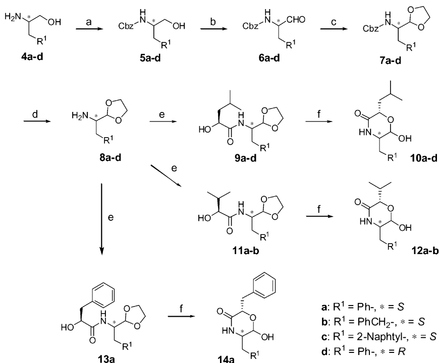
Scheme 1. Conditions: (a) Cbz-OSu, THF; (b) SO 3 /pyridine, DIPEA, DMSO/CH 2 Cl 2 ; (c) ethylene glycol, pyridinium p -toluenesulfonate, toluene; (d) Pd/C, EtOAc; (e) \alpha -hydroxy acetic acids, HOBt, Et 3 N, EDC, DMF/CH 2 Cl 2 ; (f) 6 M HCl, THF.
