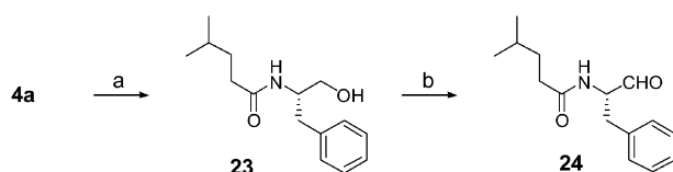
Scheme 3. Conditions: (a) 4-methylpentanoic acid, HOBT, Et_3N , EDC, DMF/ CH_2Cl_2 ; (b) SO_3 /pyridine, DIPEA, DMSO/ CH_2Cl_2 .
