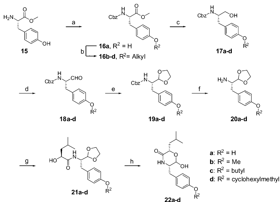
Scheme 2. Conditions: (a) Cbz-OSu, THF; (b) (CH_3)_2SO_4 , K_2CO_3 , acetone; or alkyl bromide, K_2CO_3 , DMF; (c) NaBH_4 , LiCl, THF/EtOH; (d) SO_3 /pyridine, DIPEA, DMSO/ CH_2Cl_2 ; (e) ethylene glycol, pyridinium p -toluenesulfonate, toluene; (f) Pd/C, EtOAc; (g) L-leucic acid, HOBT, Et_3N , EDC, DMF/ CH_2Cl_2 ; (h) 6 M HCl, THF.
